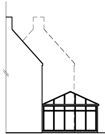
SIDE ELEVATION AS PROPOSED (1:100)
