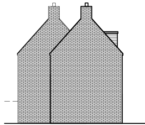
SIDE ELEVATION AS EXISTING (1:100)
