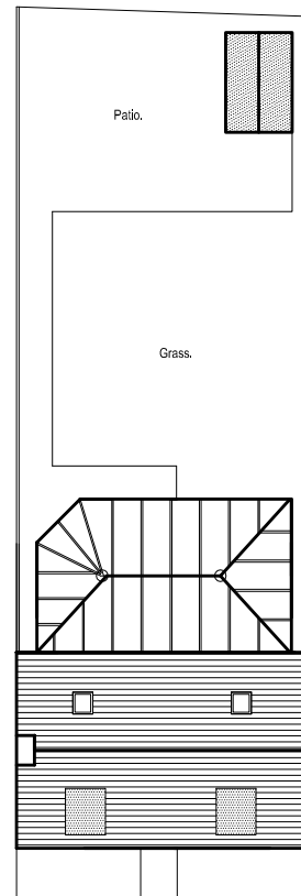
ROOF PLAN AS PROPOSED (1:200)
