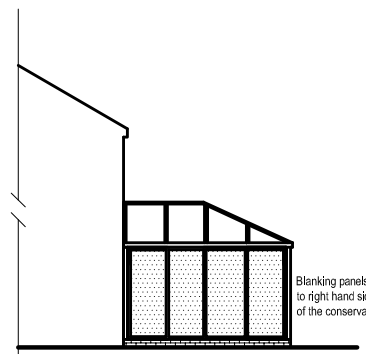
SIDE ELEVATION AS PROPOSED (1:100)
