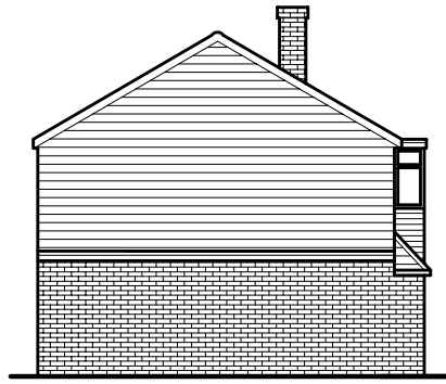
SIDE ELEVATION AS EXISTING (1:100)
